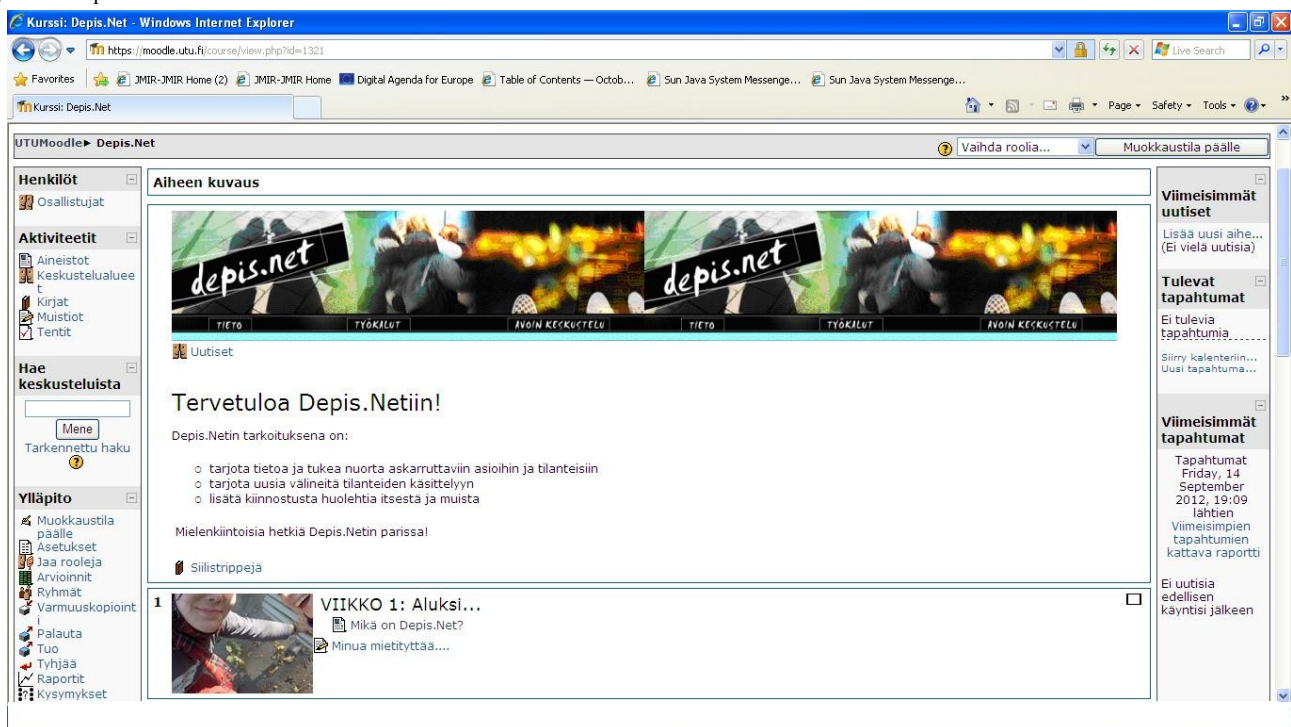
Figure 1. Depis.Net website.
